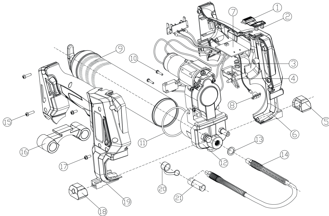
Fig. 12.-1 Exploded view of the accu grease gun
