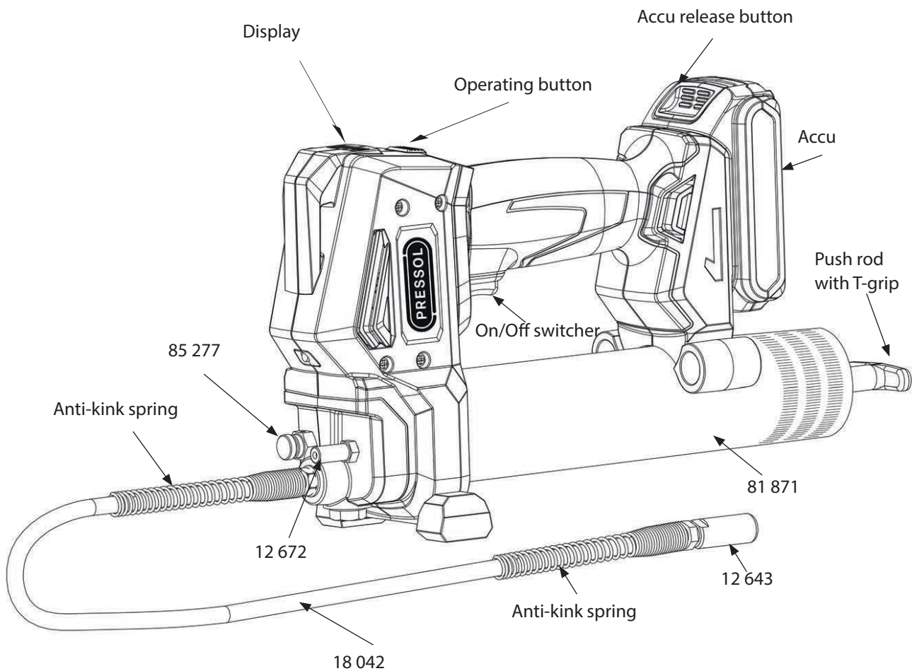
Fig. 3.2 -1: Structure accu grease gun
